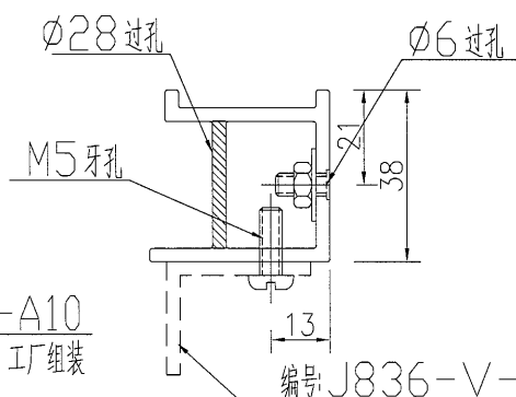
SECTION C-C
