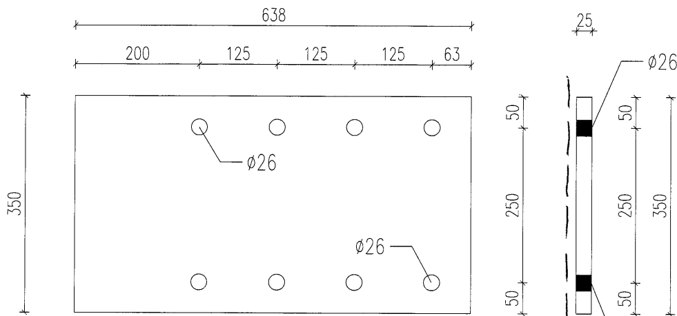
350x638x25mm THK. GMS PALTE 43.82kg/pc
