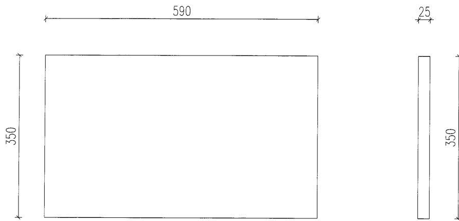
350x590x25mm THK. GMS PALTE 40.53kg/pc
