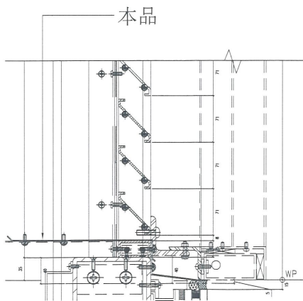
D29 SECTION DETAIL FOR ALUM LOUVER 9010
