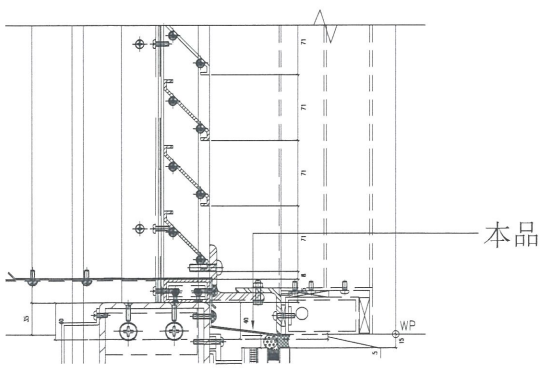
D29 SECTION DETAIL FOR ALUM LOUVER 9010
