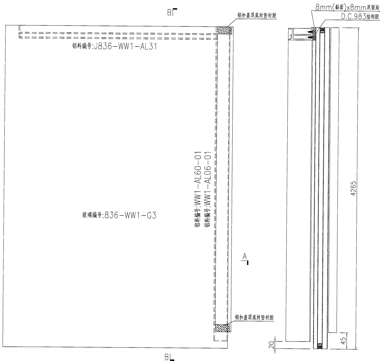
SECTION B-B
