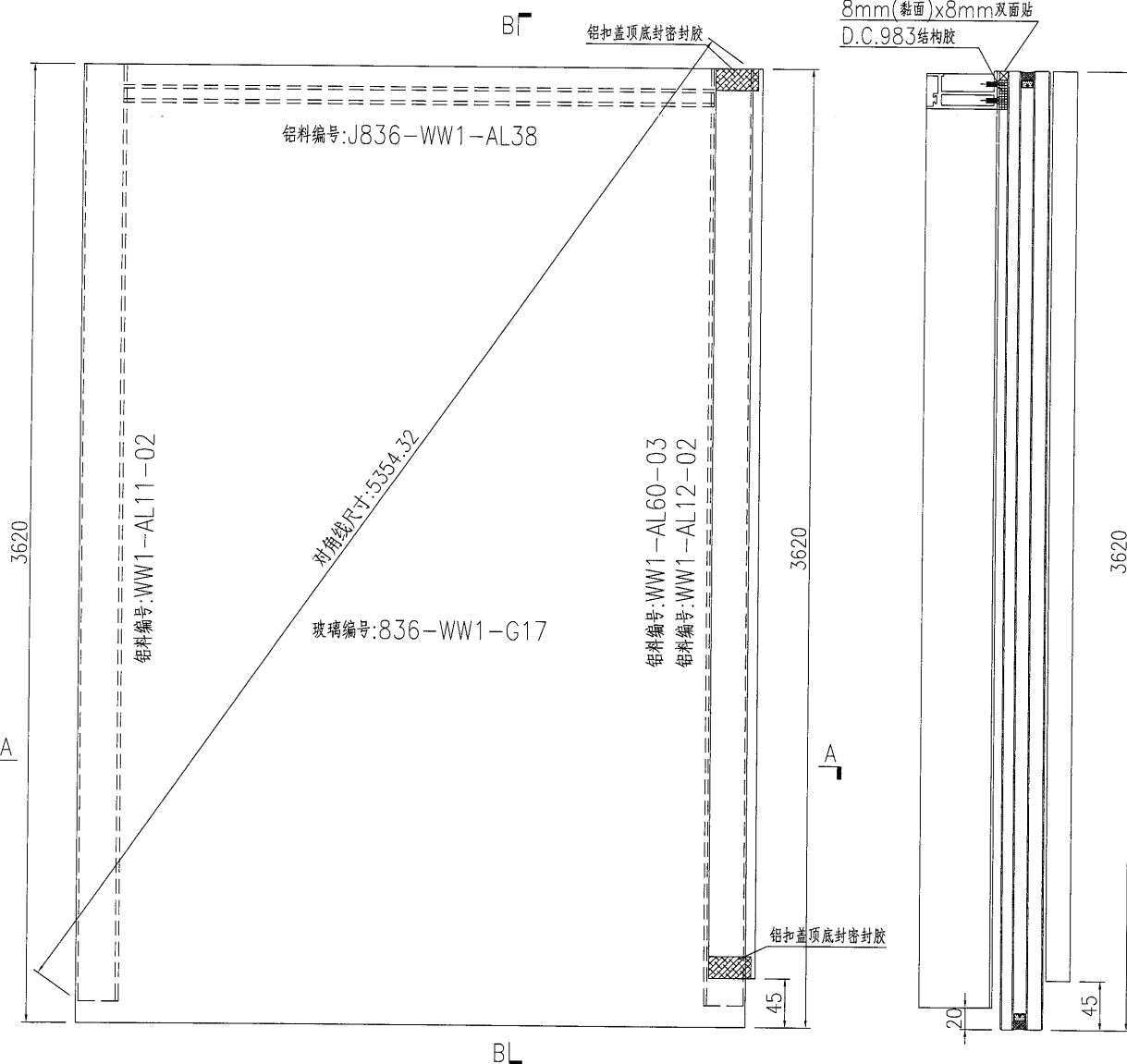
SECTION B-B
