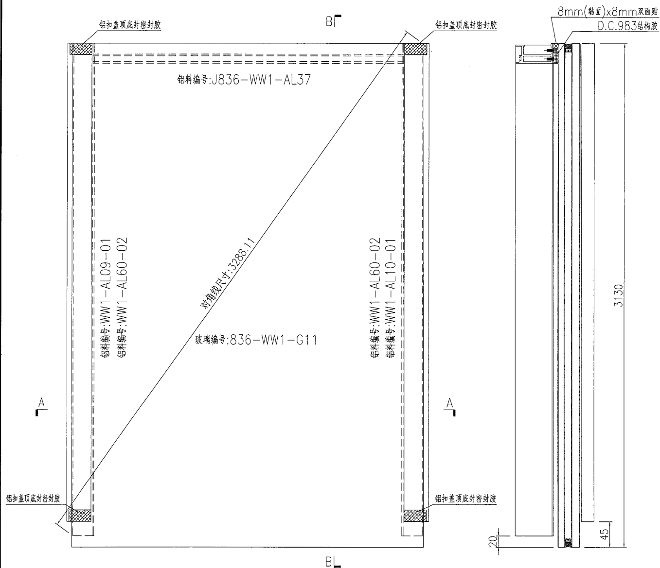
SECTION B-B
