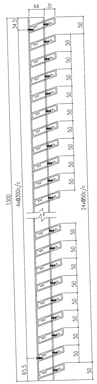
SECTION B-B
