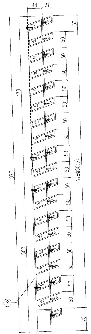
SECTION B-B
