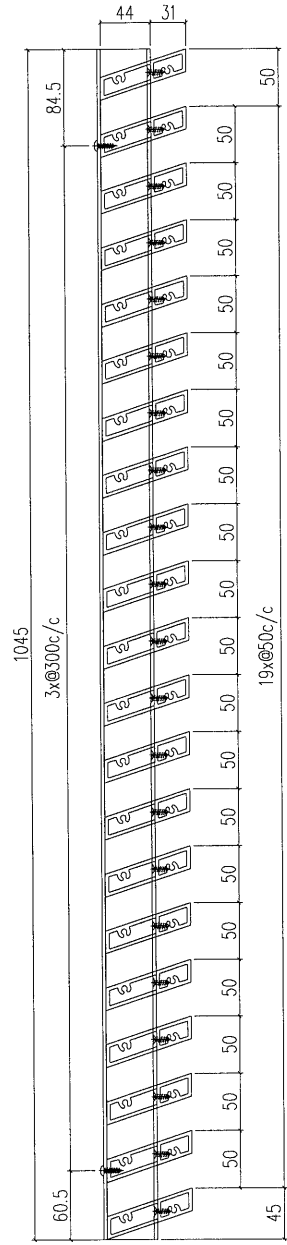
SECTION B-B
