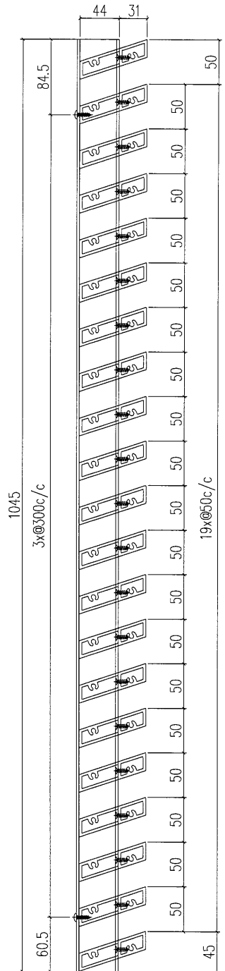
SECTION B-B
