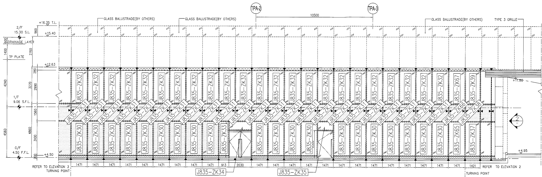
1 PARTIAL ELEVATION
