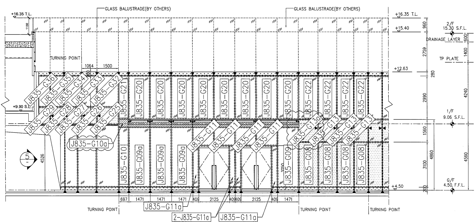
3 PARTIAL ELEVATION
