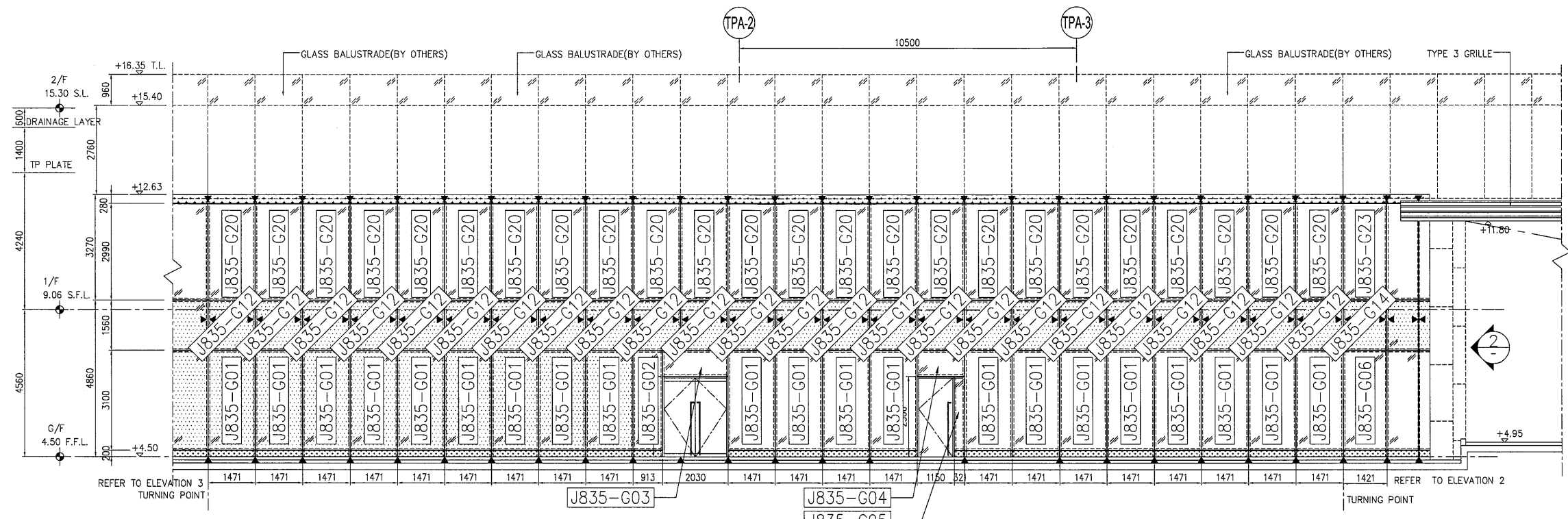
1 PARTIAL ELEVATION
