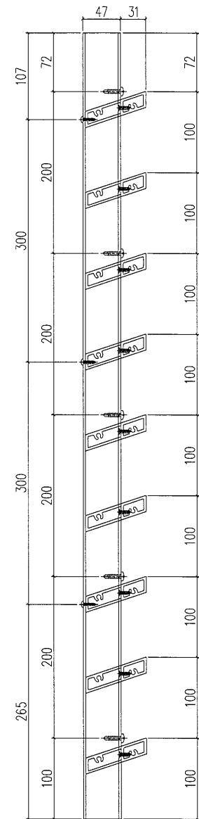
SECTION B-B
