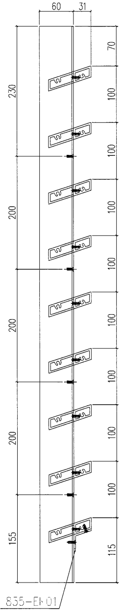
SECTION B-B
