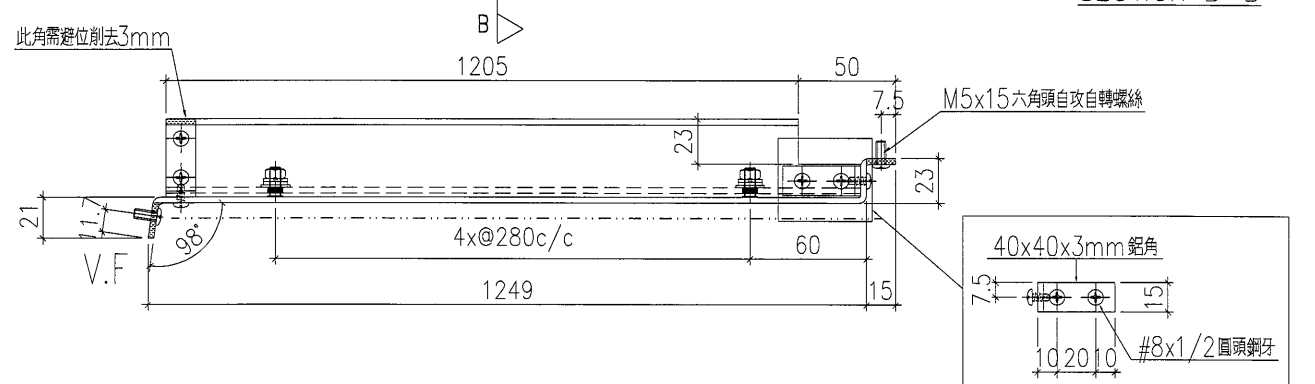
SECTION B-B
