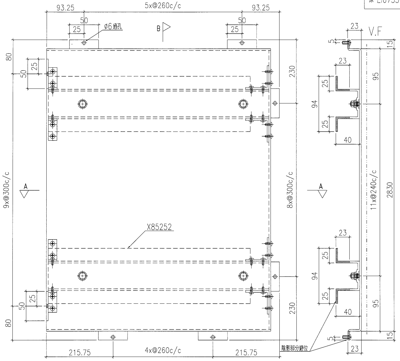
SECTION B-B
