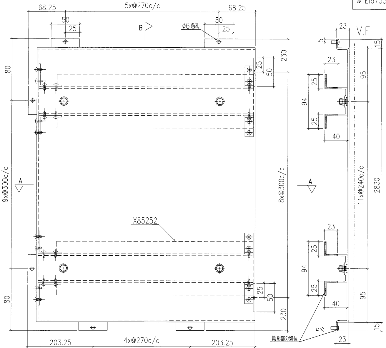
SECTION B-B
