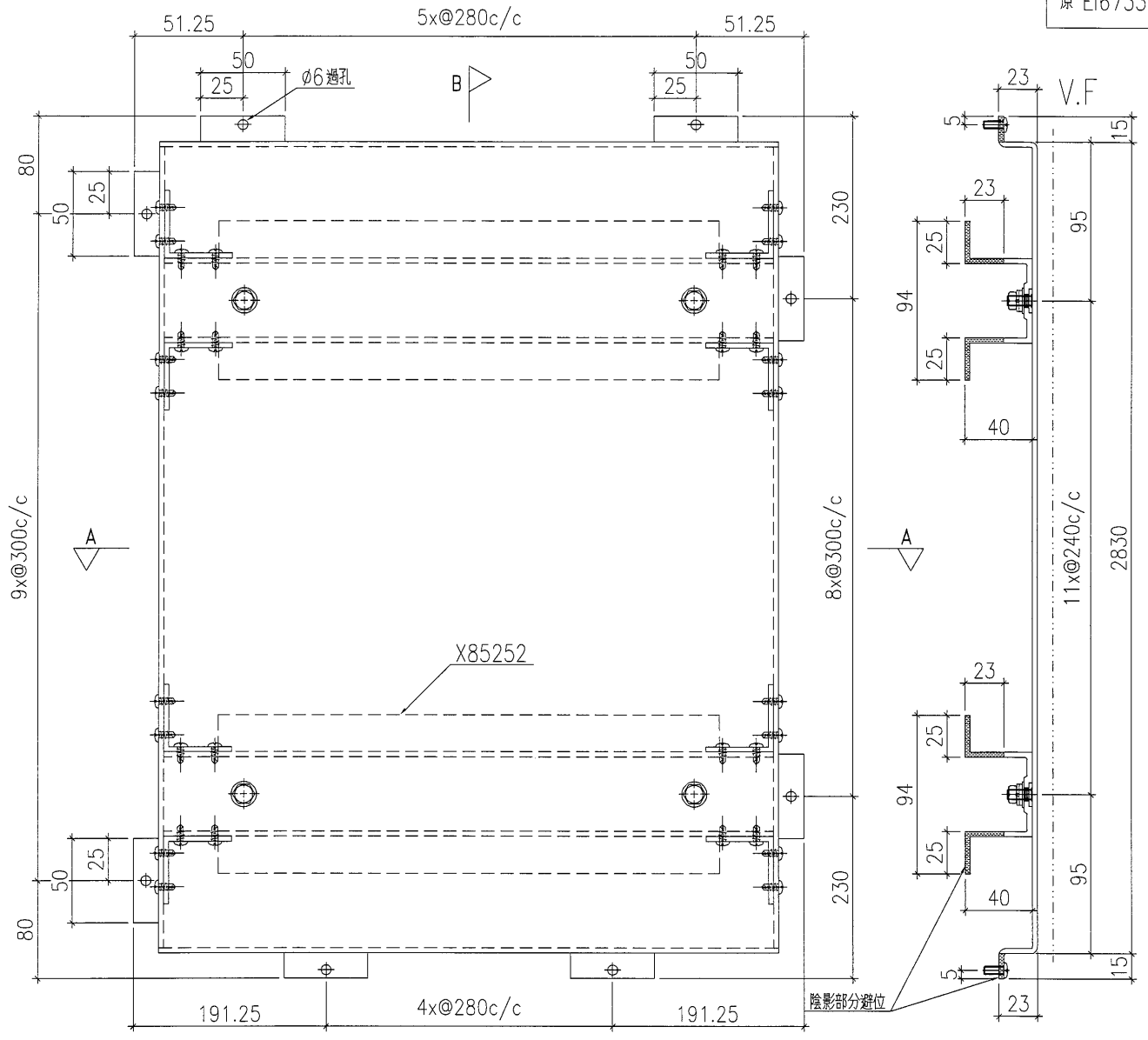
SECTION B-B
