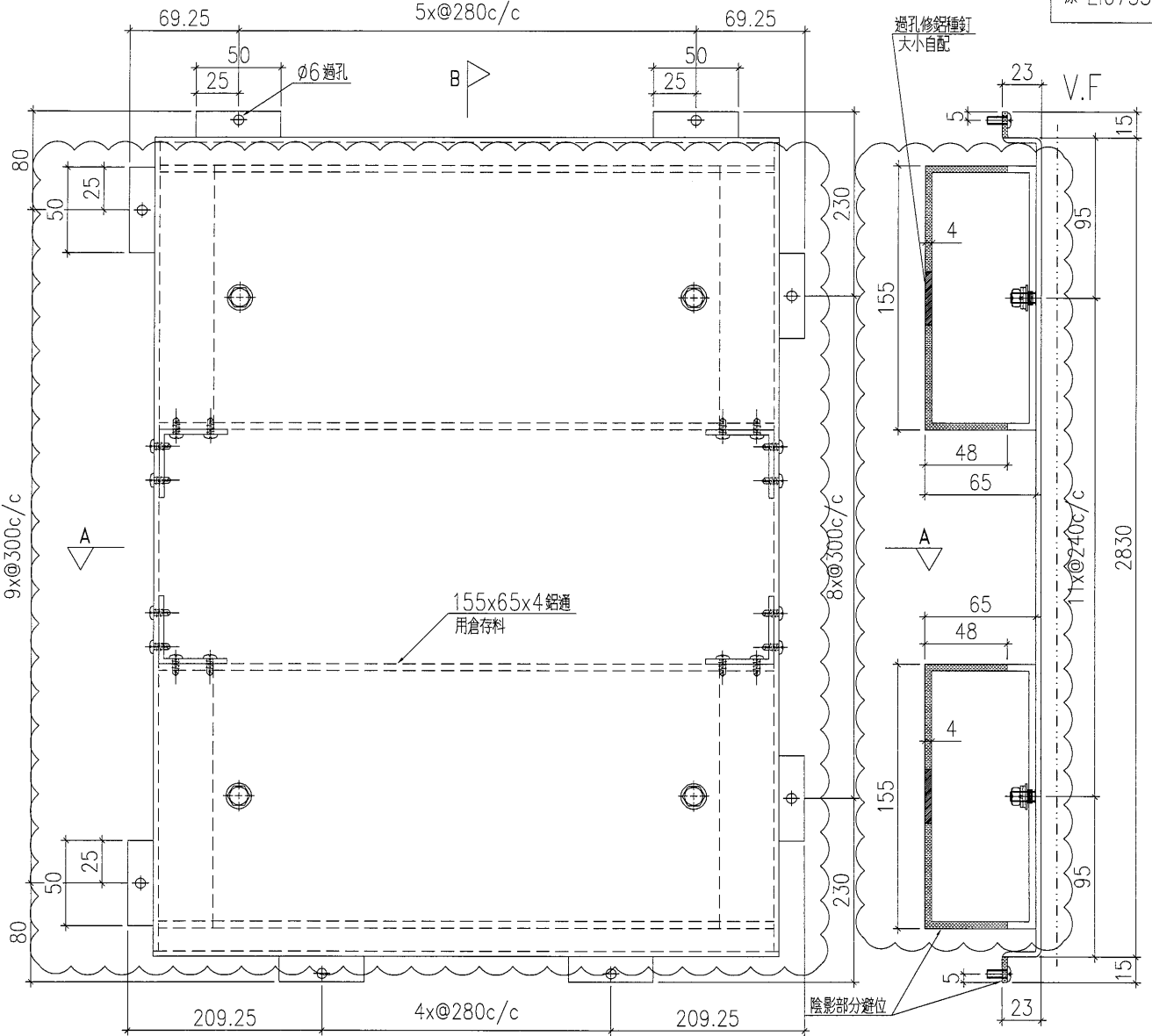
SECTION B-B
