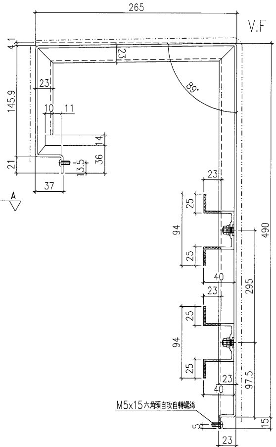
SECTION B-B
