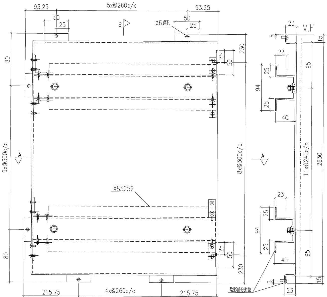
SECTION B-B
