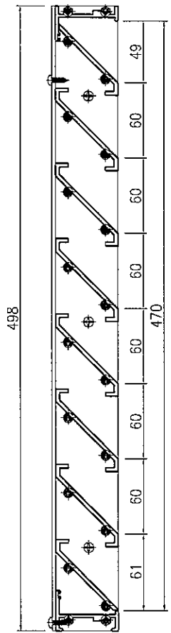
SECTION B-B
